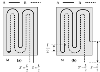
Fig. 2. Illustration of asymmetrical fiber winding. (a) CCW (denoted by A) and CW (denoted by B) wound fiber sections have the same length. (b) CWW section is short by a length of l , resulting in a shift of l/2 of the coil midpoint to the CW side.
